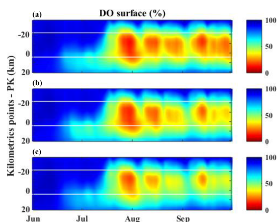
Figure 6. Spatiotemporal evolution of daily average surface DO (saturation in %) along the tidal Garonne River section for the scenarios of reference (a), combining +10 \text{ m s}^{-1} of river flow and reduction of 50 % of SO releases (b), and combining +10 \text{ m}^3 \text{ s}^{-1} of river flow, a reduction of 50 % of SO releases and urban effluent discharges at KP15 (c). The y axis represents the kilometric points, and the white lines represent Bordeaux and Portets.
